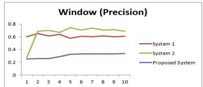
Fig. 24: Window (Precision)
