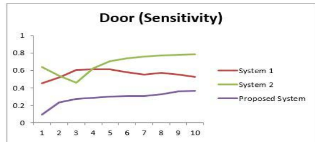
Fig. 16: Door (Sensitivity)
