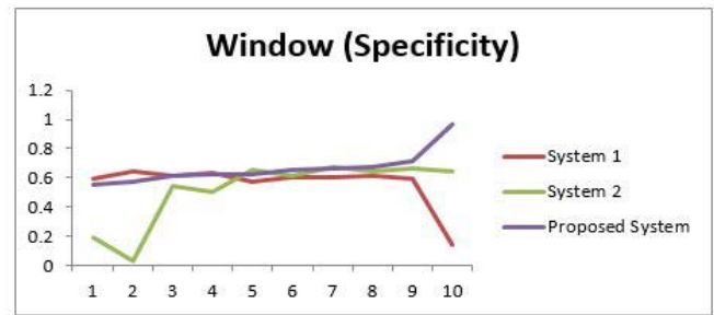
Fig. 23: Window (Specificity)
